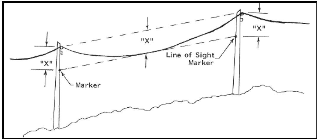
Figure 1 – Line of Sight Method of Sagging Conductors
