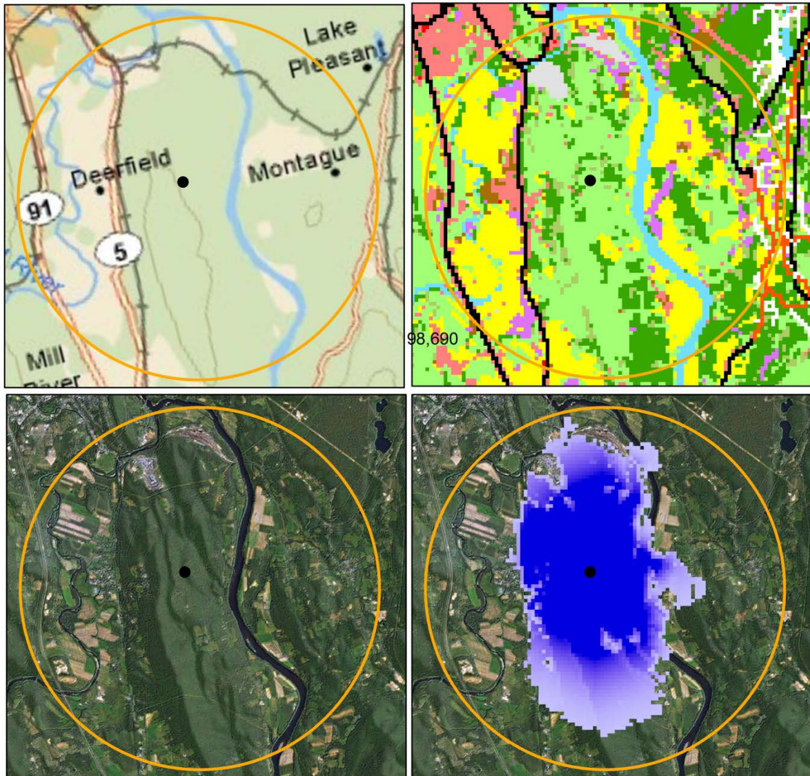
Figure 2: Detailed look at Kernel B in Figure 1. The top left image shows the topographic map for a rough location. The top right shows detail of the land use grid. The bottom left shows the aerial and the 3km circular resistant kernel distance. The bottom right shows the kernel spread. Kernel B is constrained on the west by roads and railroads and on the east by water. The kernel can flow well through the natural landscape in the north and south direction.
