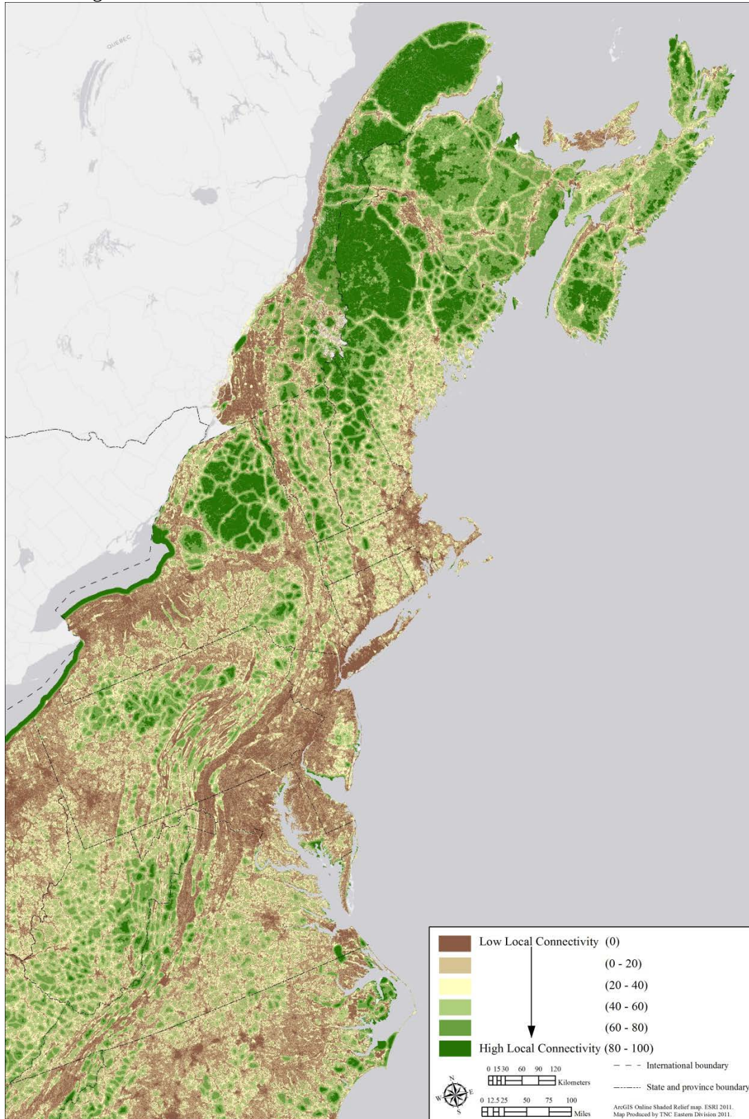
Map 1: Local connectedness. This map estimates the degree of connectedness of a cell with its surroundings within a three kilometer radius.
