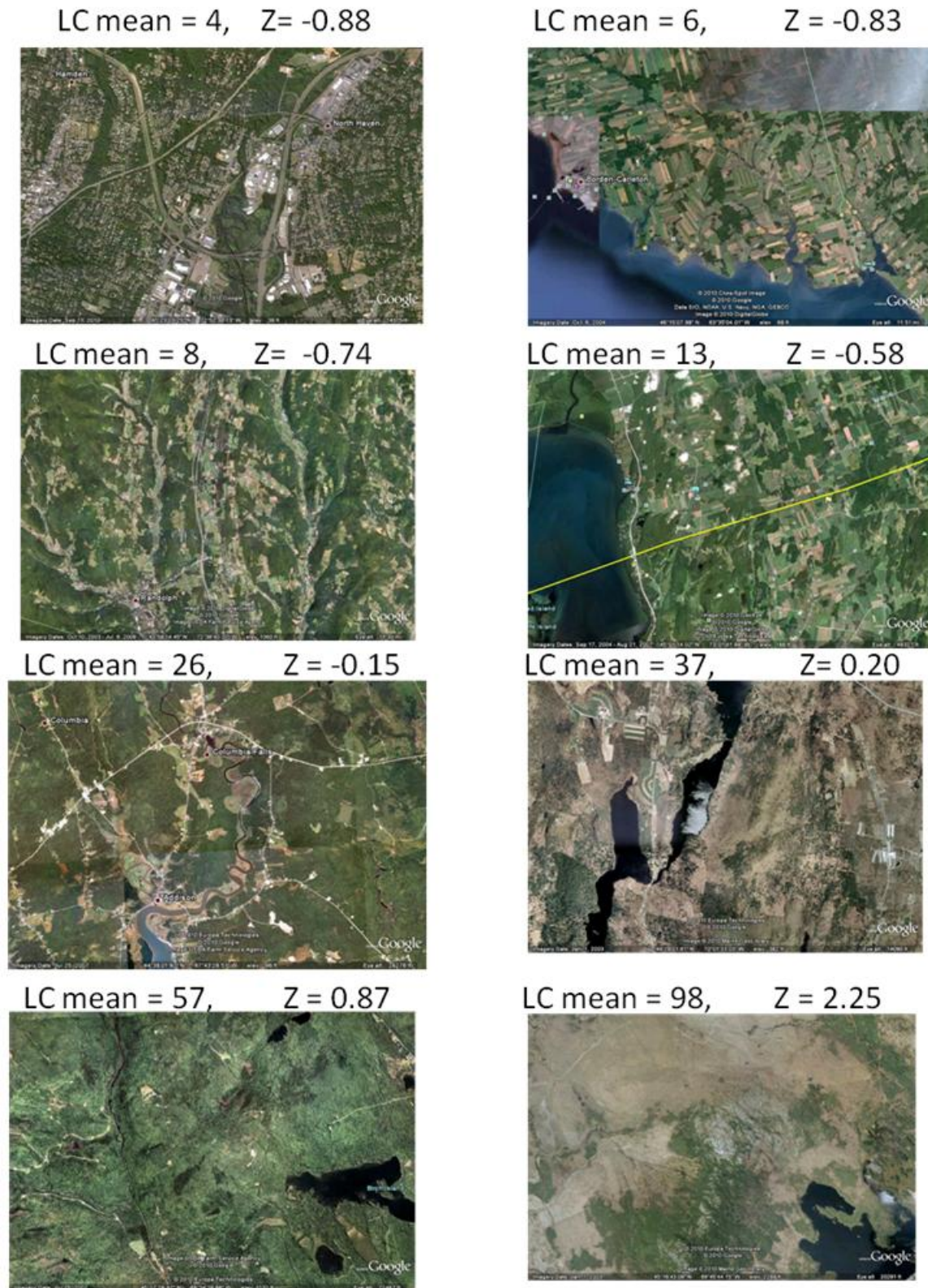
Figure 3: A gallery of satellite images and their corresponding local connectedness (lc) scores. The mean scores are based on a roughly circular site positioned at the center of each image (not shown). Z is units of standard deviation from the regional mean.
