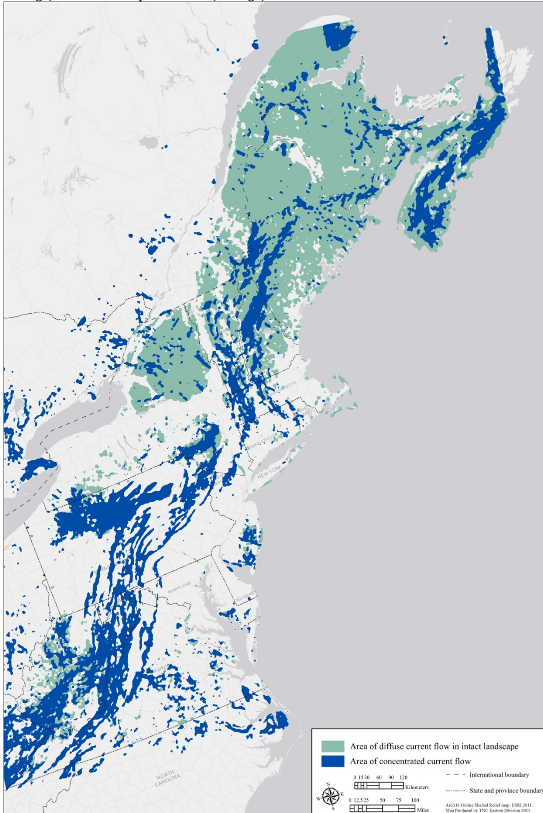
Map 3: Grouped regional flow patterns. This map shows areas of concentrated flow (above average), diffuse or dispersed flow (average).
