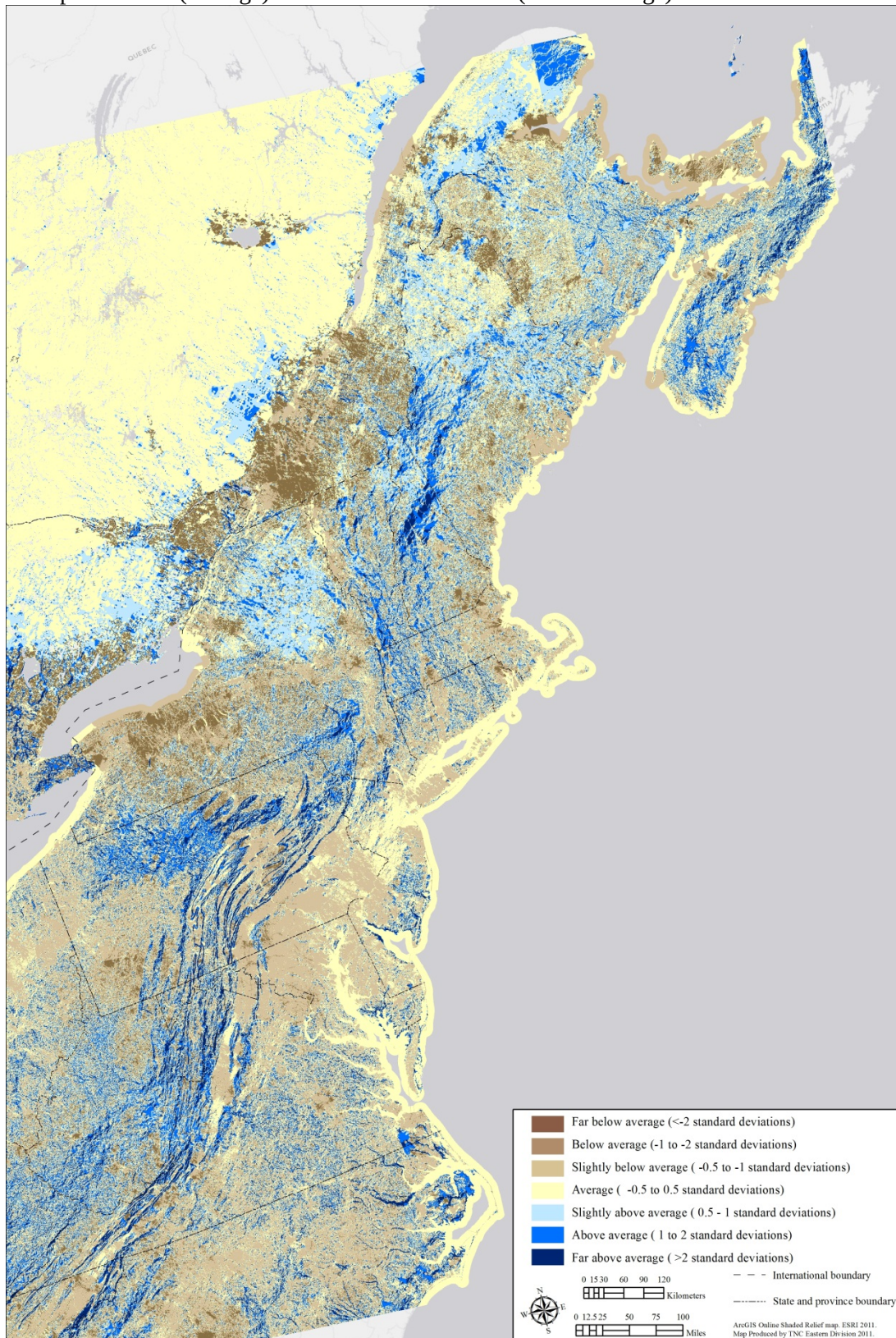
Map 2: Regional flow patterns. This map shows areas of concentrated flow (above average), diffuse or dispersed flow (average) and low or blocked flow (below average).
