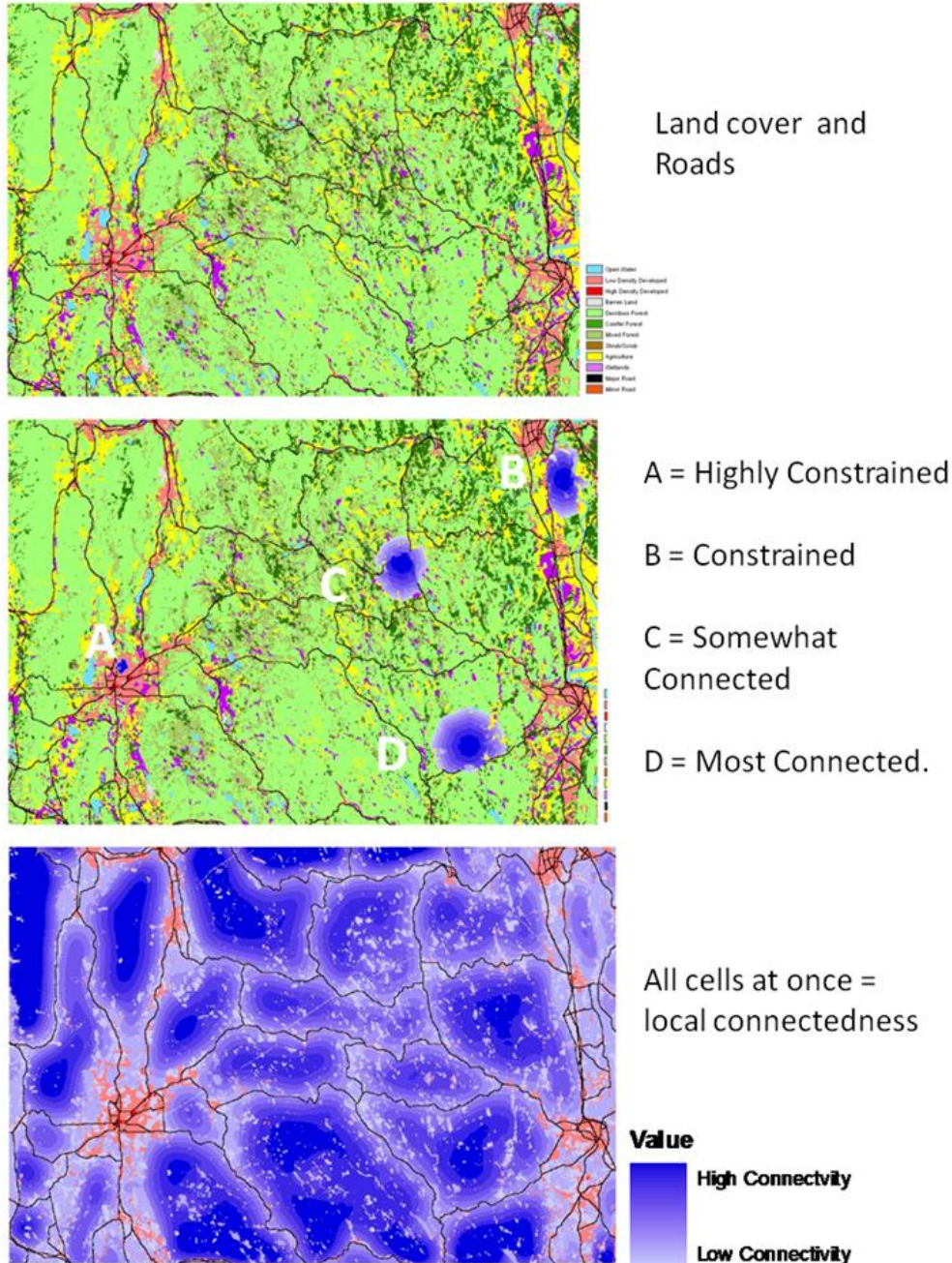
Figure 1: Examples of four resistant kernel cells shown against the land cover and roads map. The focal cell is the central point of each kernel and the spread, or size, of the kernel is the amount of constraints, so the score for the focal cell reflects the area around the cell. Kernel A is the most constrained; D is the least constrained.
