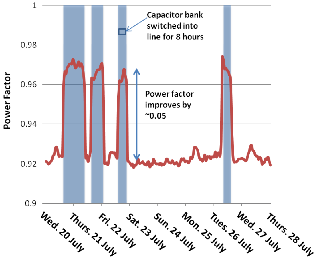
Figure 14. Example of Automated Capacitor Bank Control
