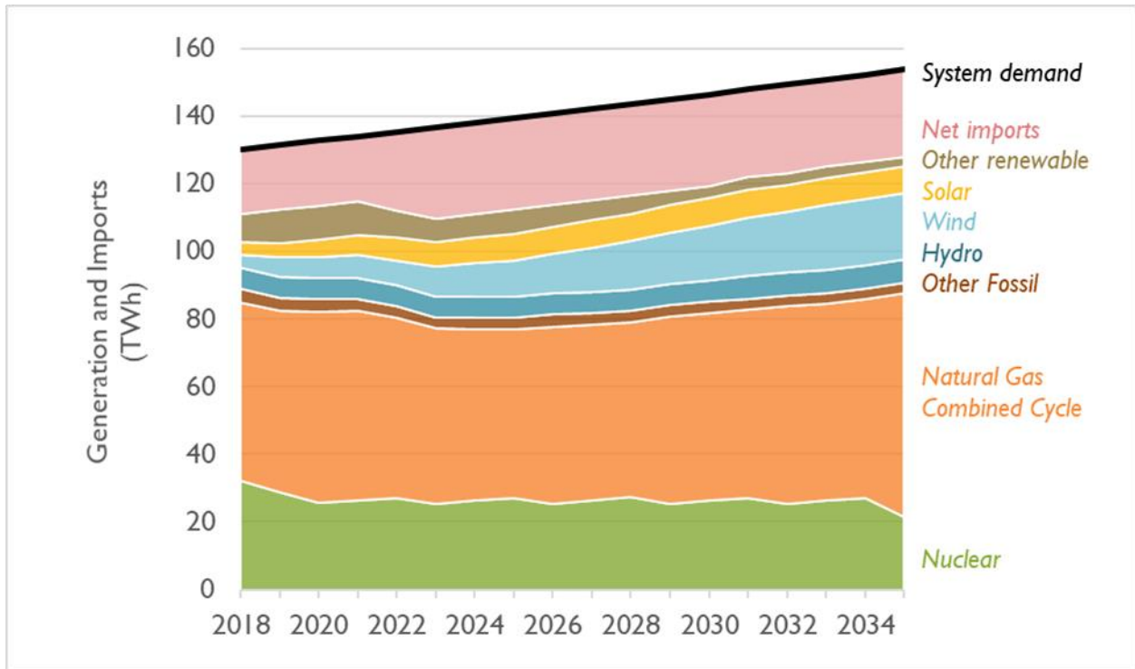
Figure 25. AESC 2018 New England-wide generation, imports, and system demand
